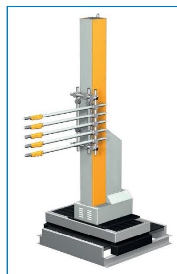
Robot d'application Reciprocator with guns
